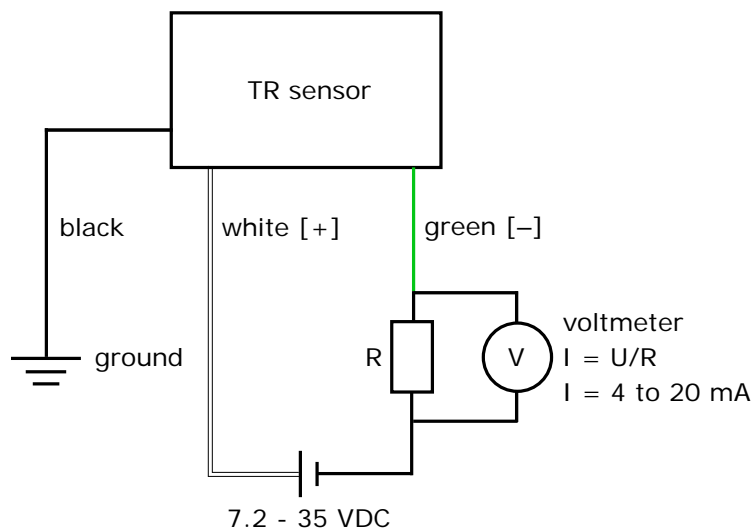
Figure 8.3.3 Electrical diagram of the connection of LP02-TR to a typical voltmeter or datalogger with the capacity to measure voltage signals. Usually a 100\ \Omega shunt resistor ( R ) is used to convert the current to a voltage. LP02-TR operates on a supply voltage of 7.2 to 35 VDC.
