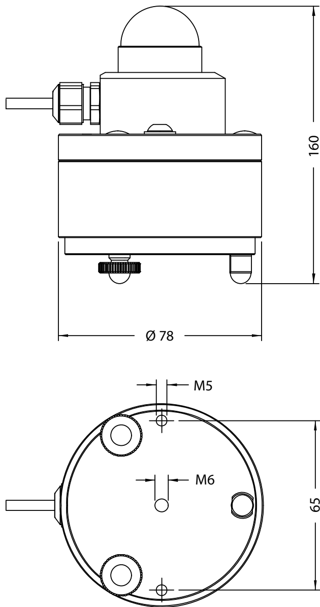
Figure 8.2.2 Dimensions of LP02-TR in 10^{-3} m
